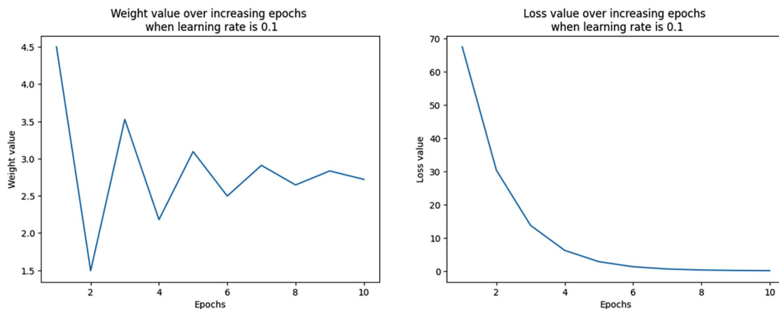
Figure 1.21: Weight & loss values over increasing epochs when learning rate is 0.1
